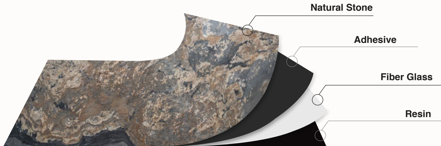
Composition of skin Flexible Slate Veneer
